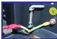
Earthing cable
